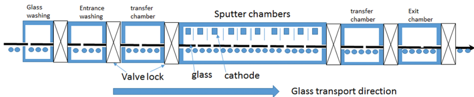
Figure 7. Schematic of a continuous-batch sputter-coating reactor, simplified from Ref. [13].
