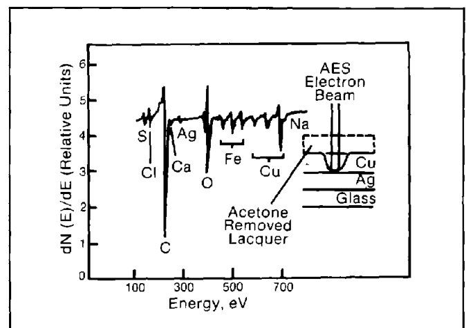
Figure 3-4b Elements Present on Copper Surface (Zero Time) Shown Using an AES Scan (Thomas 1983)
