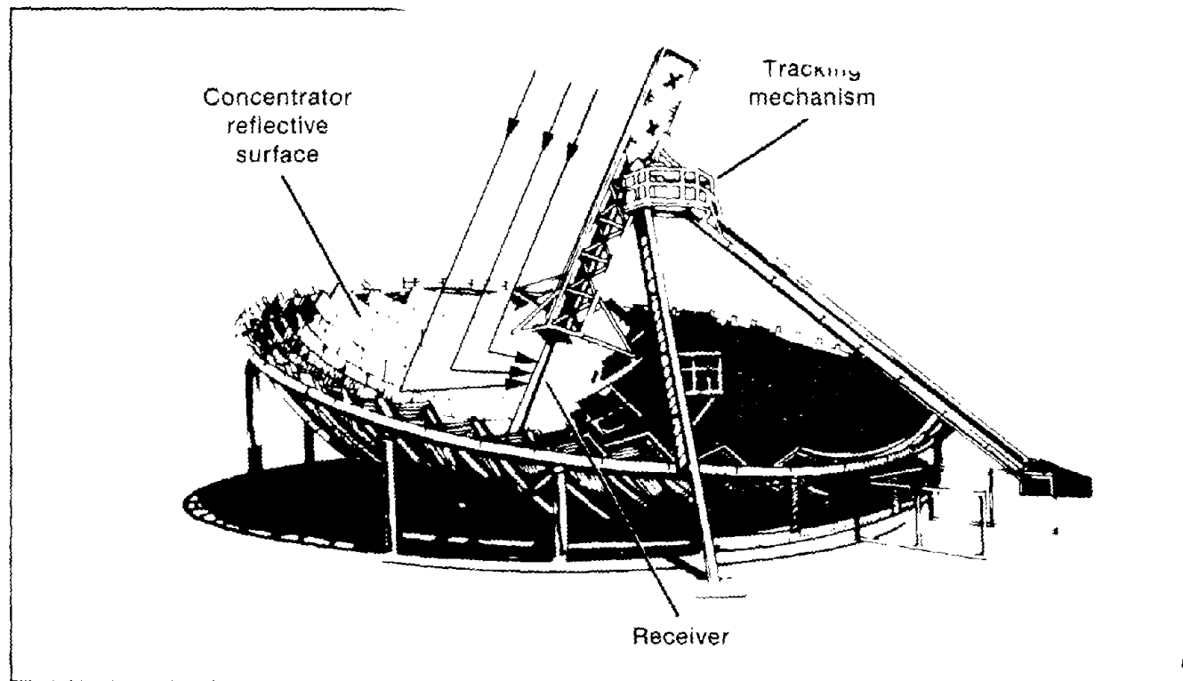
Figure 1-3 Spherical Bowl
