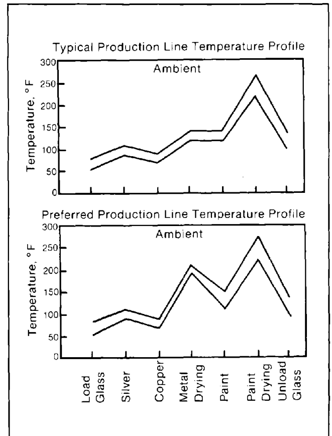
Figure 5-10 Production-Line Temperature Profiles (Lind et al. 1979)
