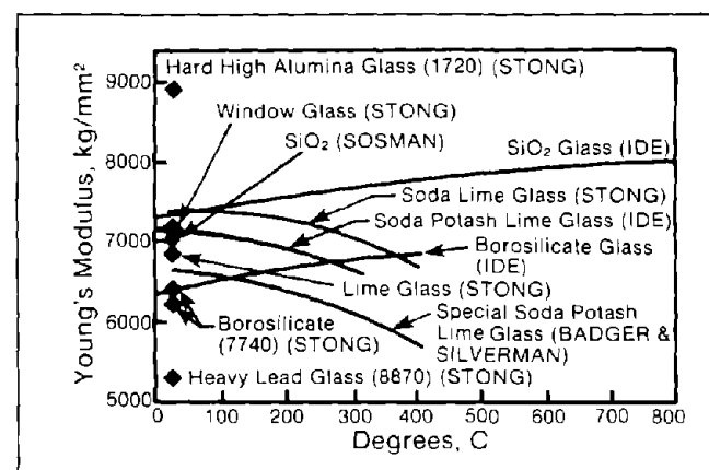
Figure 2-6 Young's Modulus of Various Glasses (Bouquet 1979)
