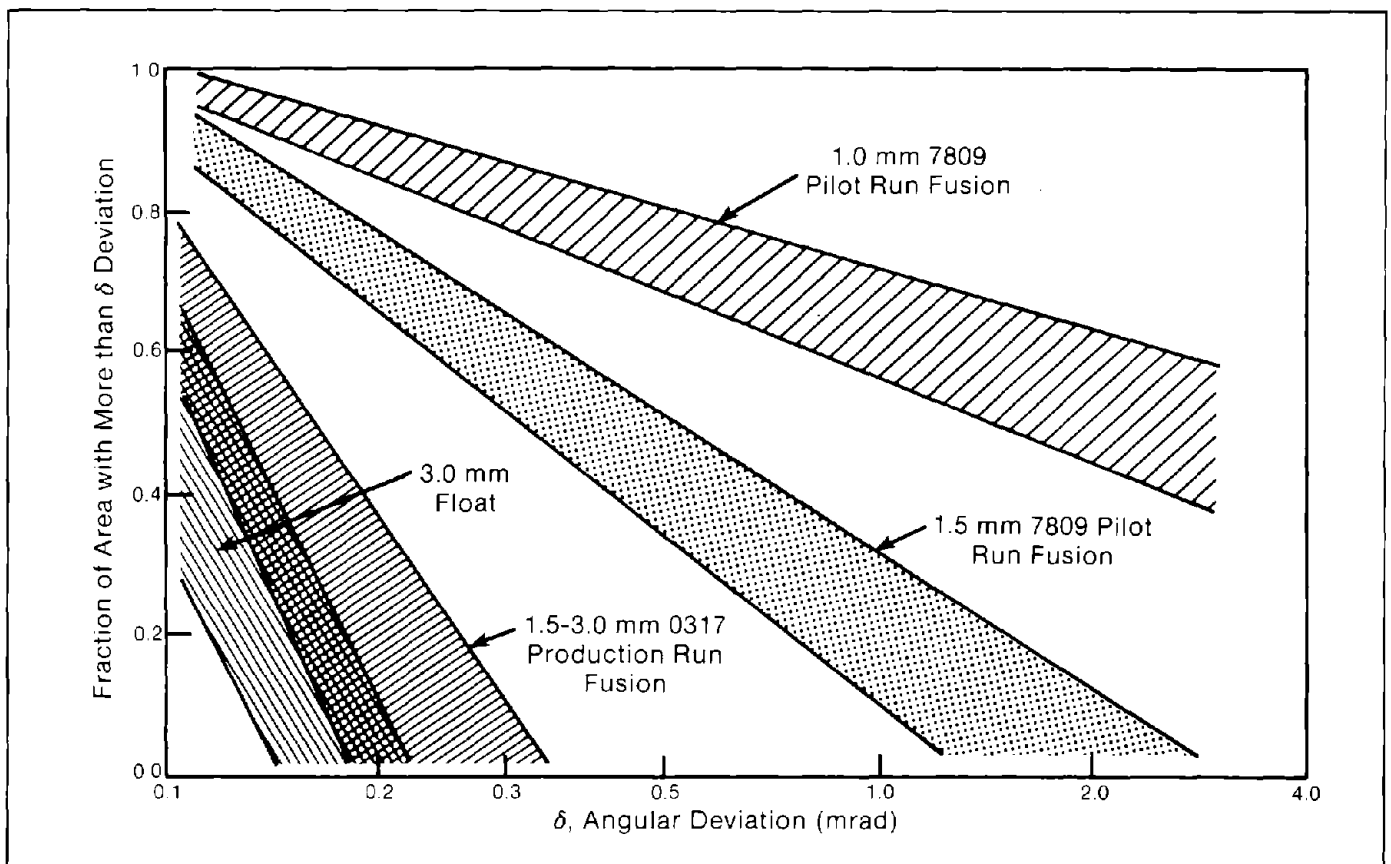
Figure 2-19 Fraction of Glass Surface Area with More than Angular Deviation from Specular Reflection (Coyle and Livingston 1981)
