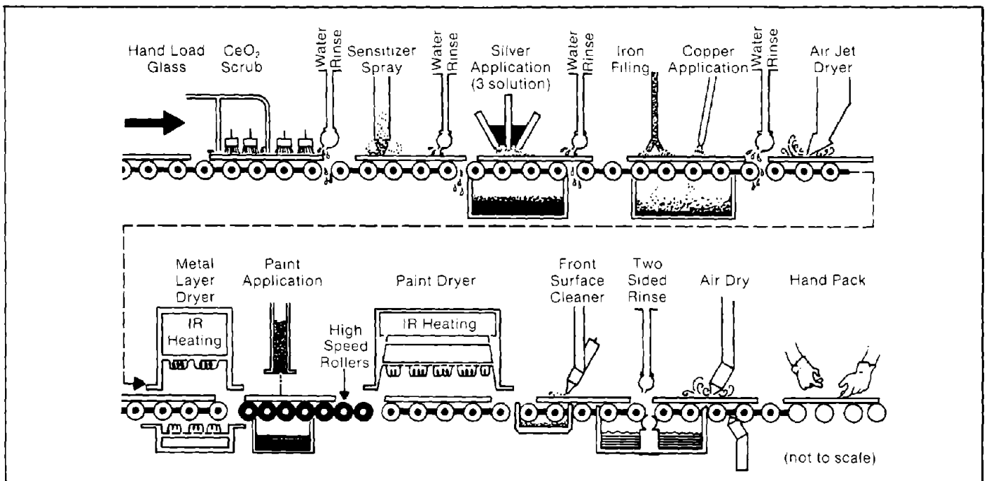
Figure 5-2 Wet-Chemistry Mirror Production Sequence (Lind et al. 1979)
