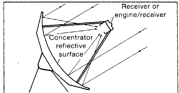
Figure 1-2 Parabolic Dish
