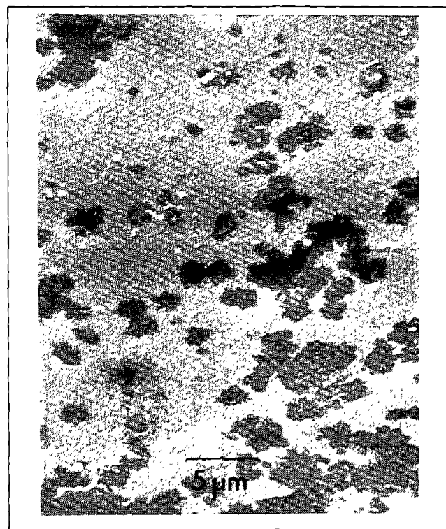
Figure 3-7 Scanning Electron Micrograph of a Field-Corroded Mirror (Vitko 1982)
