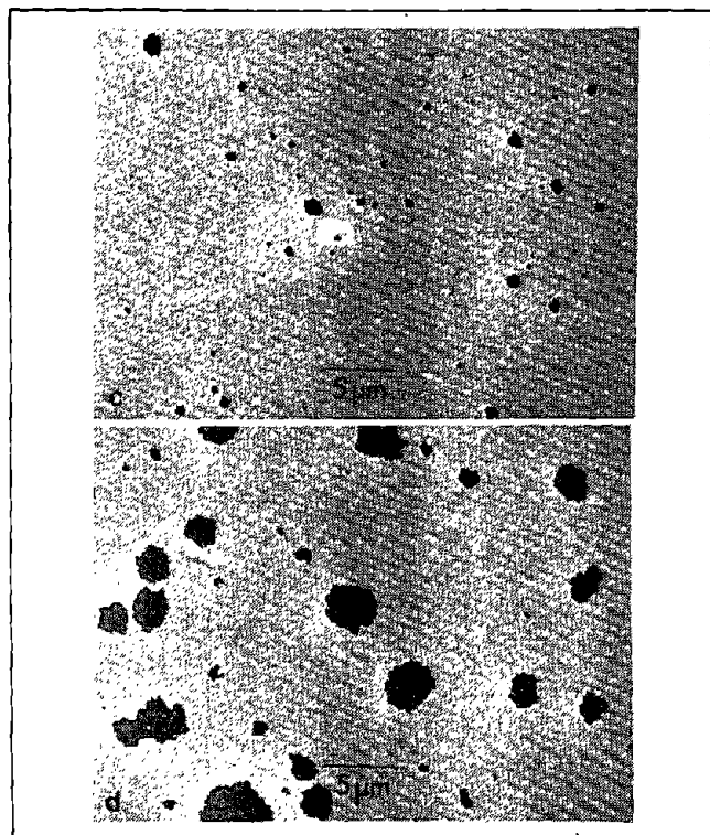
Figure 3-6 Scanning Electron Micrographs of Silver Films on Float Glass Exposed to 1000 ml of Distilled Water at 90°C (Vitko 1982)
