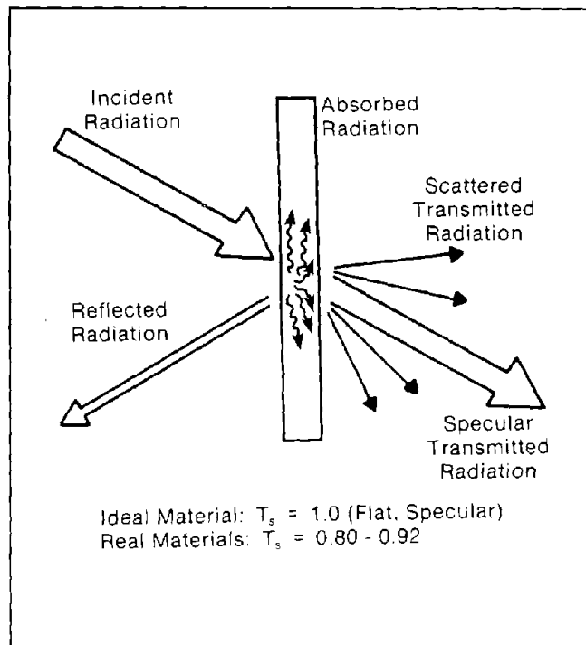
Figure 2-1 Optical Properties of Transmitters (Lind 1981)
